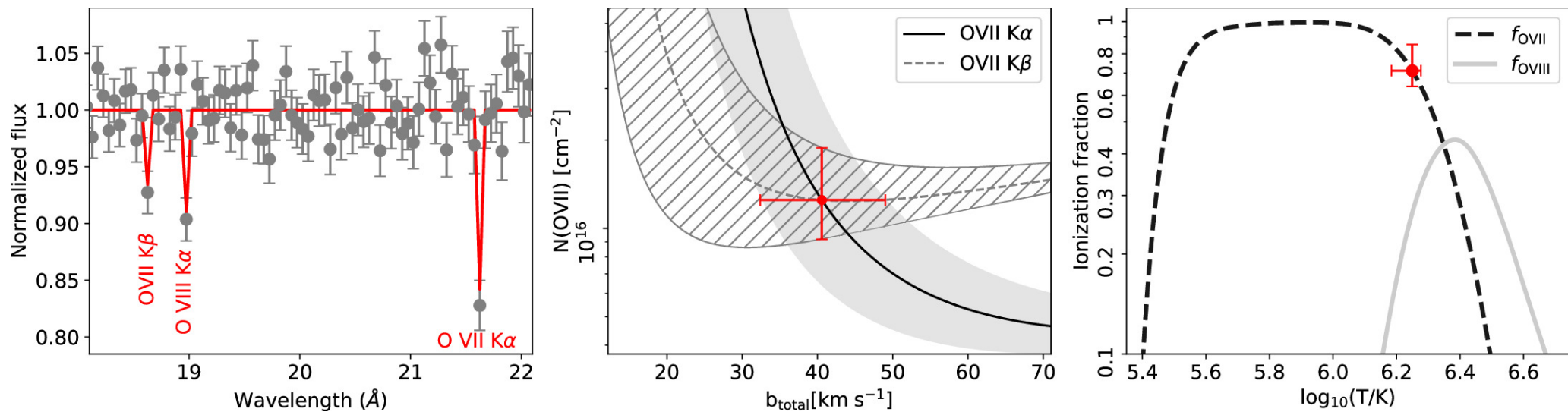
Figure 1. from Sanskriti Das 2024 Astrophys. J. Lett. 963 doi:10.3847/2041-8213/ad2a43 https://dx.doi.org/10.3847/2041-8213/ad2a43 © 2024. The Author(s). Published by the American Astronomical Society.
