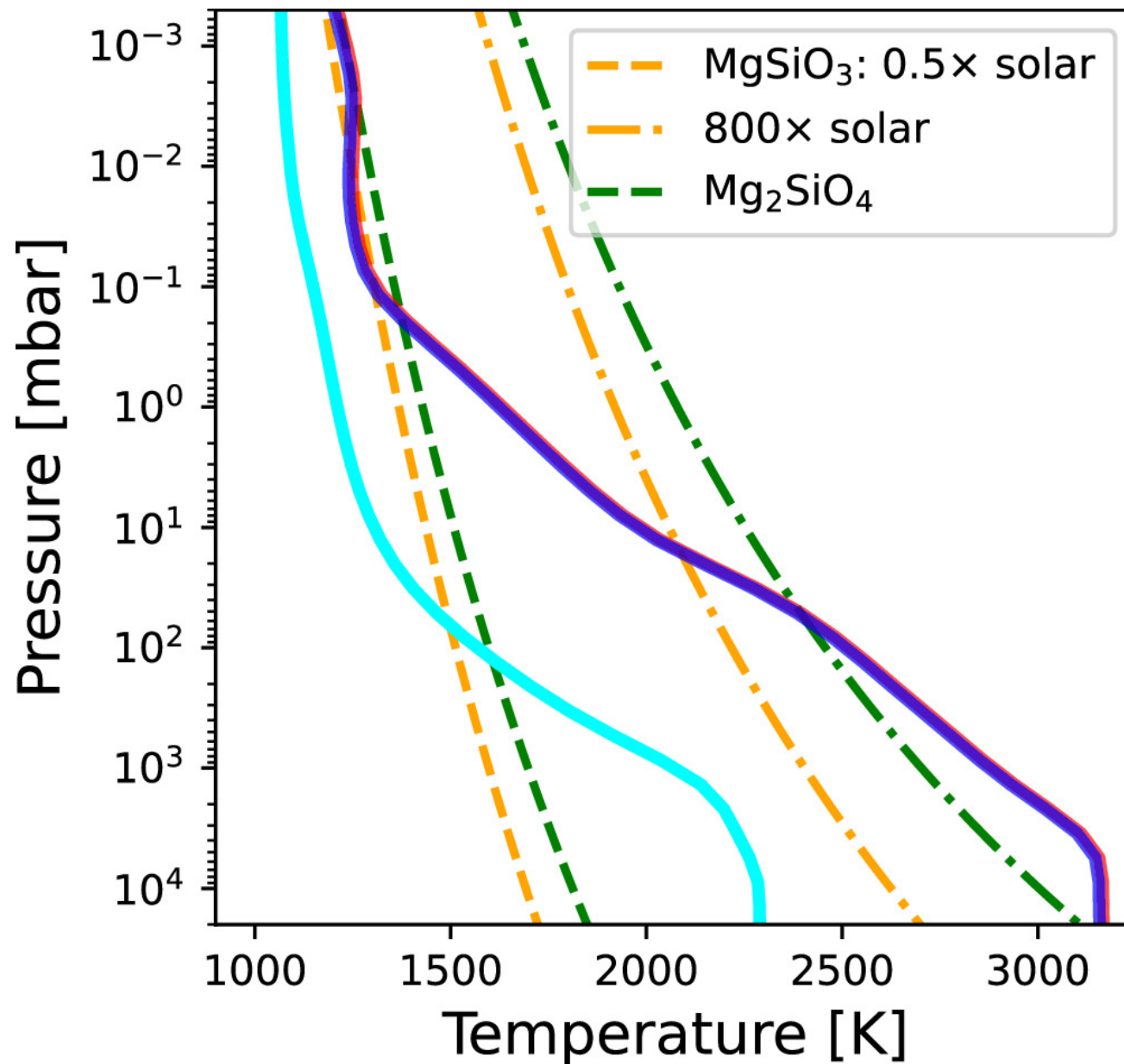
Figure 5. from Michael Radica et al 2024 Astrophys. J. Lett. 962 doi:10.3847/2041-8213/ad20e4 https://dx.doi.org/10.3847/2041-8213/ad20e4 © 2024. The Author(s). Published by the American Astronomical Society.
