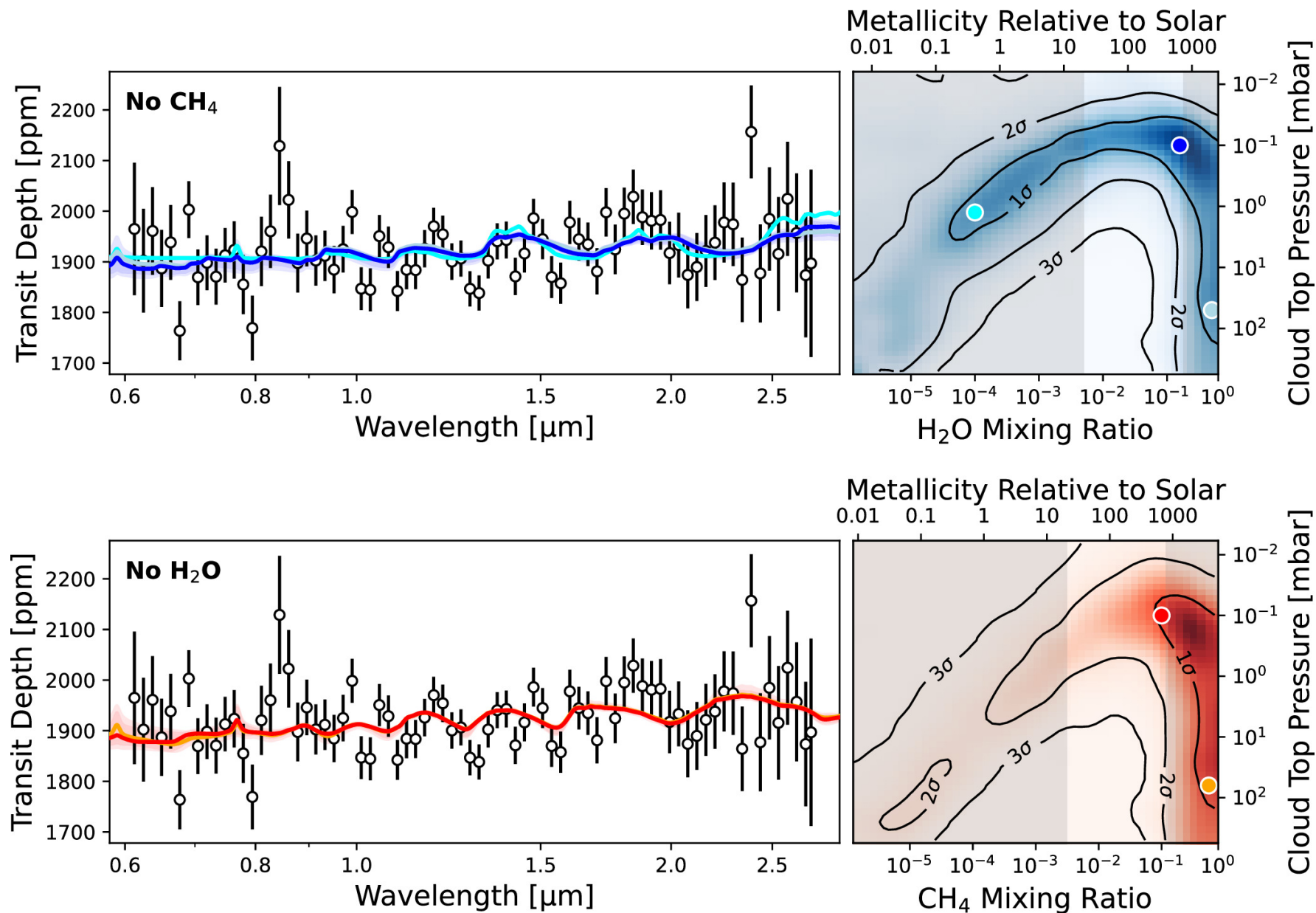
Figure 4. from Michael Radica et al 2024 Astrophys. J. Lett. 962 doi:10.3847/2041-8213/ad20e4 https://dx.doi.org/10.3847/2041-8213/ad20e4 © 2024. The Author(s). Published by the American Astronomical Society.
