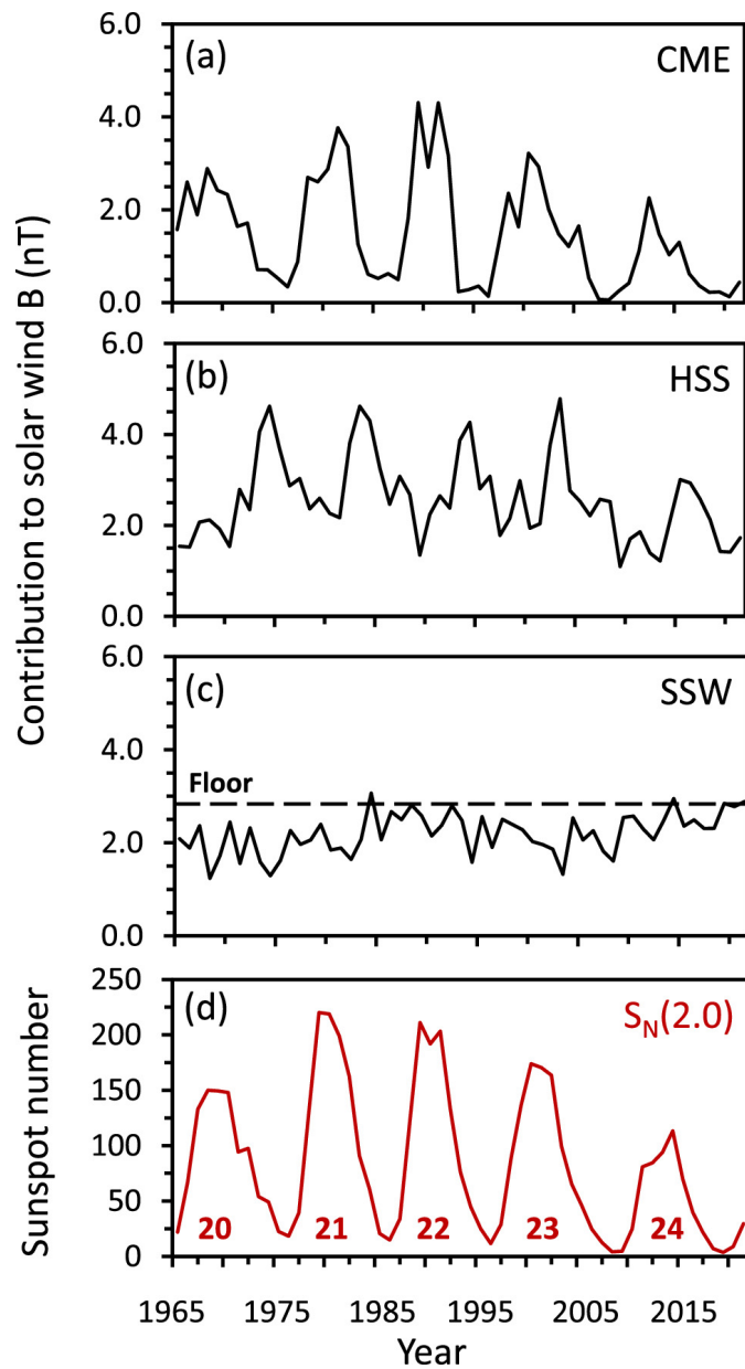
Figure 6. from E. W. Cliver et al 2024 Astrophys. J. Lett. 961 doi:10.3847/2041-8213/ad192e https://dx.doi.org/10.3847/2041-8213/ad192e © 2024. The Author(s). Published by the American Astronomical Society.
