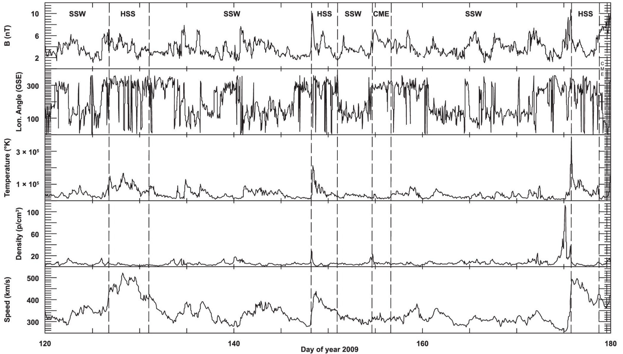
Figure 5. from E. W. Cliver et al 2024 Astrophys. J. Lett. 961 doi:10.3847/2041-8213/ad192e https://dx.doi.org/10.3847/2041-8213/ad192e © 2024. The Author(s). Published by the American Astronomical Society.
