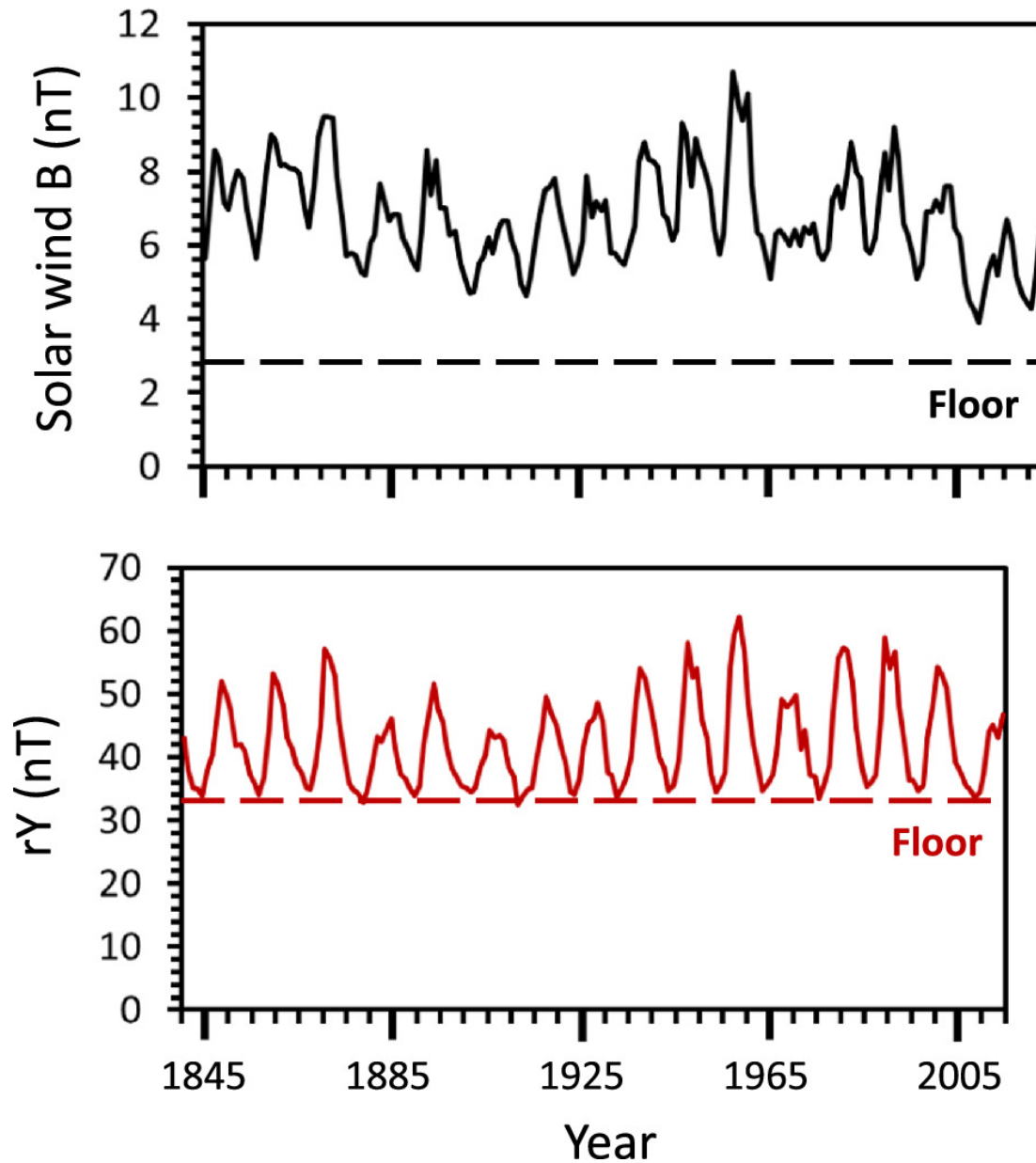
Figure 4. from E. W. Cliver et al 2024 Astrophys. J. Lett. 961 doi:10.3847/2041-8213/ad192e https://dx.doi.org/10.3847/2041-8213/ad192e © 2024. The Author(s). Published by the American Astronomical Society.
