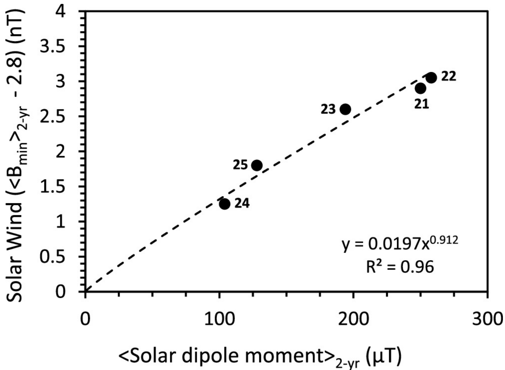
Figure 3. from E. W. Cliver et al 2024 Astrophys. J. Lett. 961 doi:10.3847/2041-8213/ad192e https://dx.doi.org/10.3847/2041-8213/ad192e © 2024. The Author(s). Published by the American Astronomical Society.
