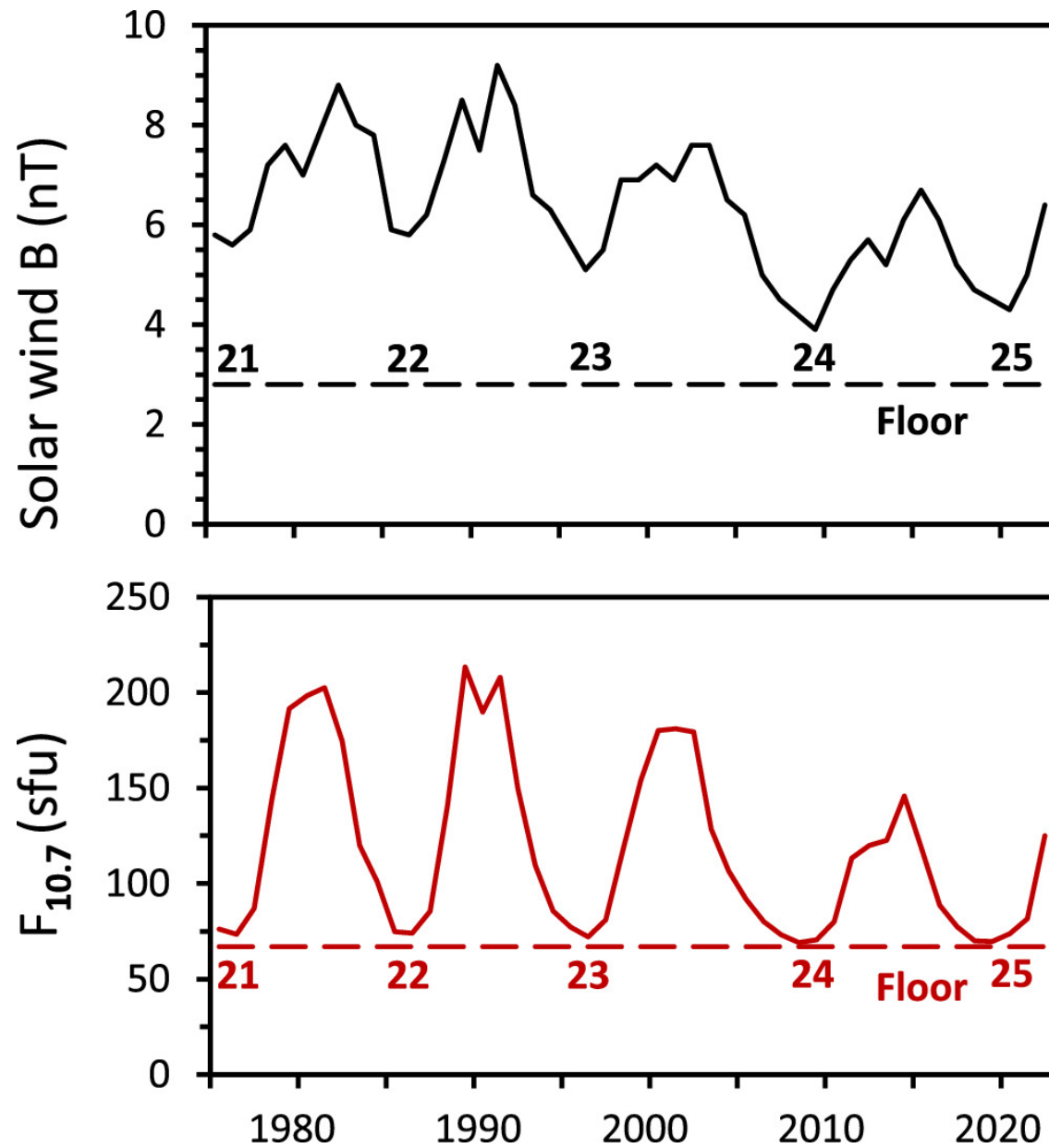
Figure 2. from E. W. Cliver et al 2024 Astrophys. J. Lett. 961 doi:10.3847/2041-8213/ad192e https://dx.doi.org/10.3847/2041-8213/ad192e © 2024. The Author(s). Published by the American Astronomical Society.
