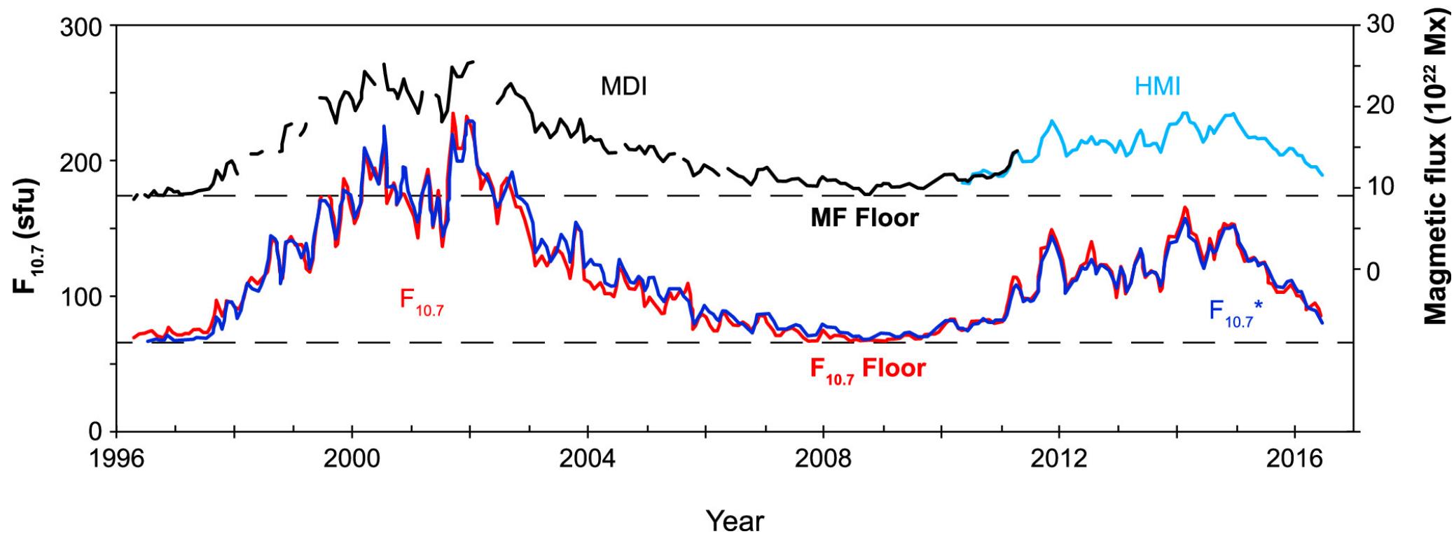
Figure 1. from E. W. Cliver et al 2024 Astrophys. J. Lett. 961 doi:10.3847/2041-8213/ad192e https://dx.doi.org/10.3847/2041-8213/ad192e © 2024. The Author(s). Published by the American Astronomical Society.
