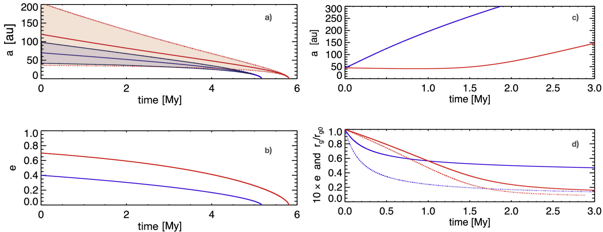
Figure 5. from Alex Doner et al 2024 Astrophys. J. Lett. 961 doi:10.3847/2041-8213/ad18b0 https://dx.doi.org/10.3847/2041-8213/ad18b0 © 2024. The Author(s). Published by the American Astronomical Society.
