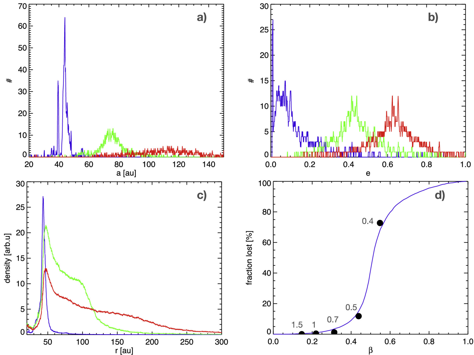
Figure 4. from Alex Doner et al 2024 Astrophys. J. Lett. 961 doi:10.3847/2041-8213/ad18b0 https://dx.doi.org/10.3847/2041-8213/ad18b0 © 2024. The Author(s). Published by the American Astronomical Society.
