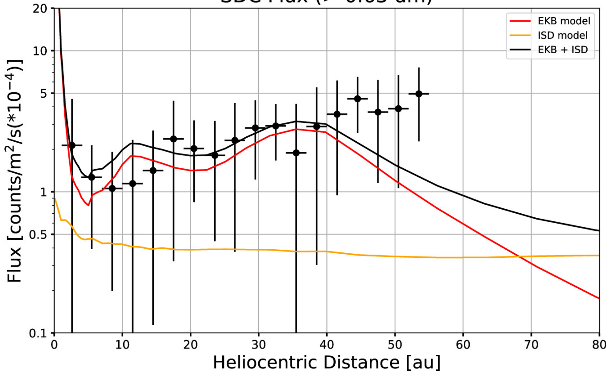
Figure 3. from Alex Doner et al 2024 Astrophys. J. Lett. 961 doi:10.3847/2041-8213/ad18b0 https://dx.doi.org/10.3847/2041-8213/ad18b0 © 2024. The Author(s). Published by the American Astronomical Society.
