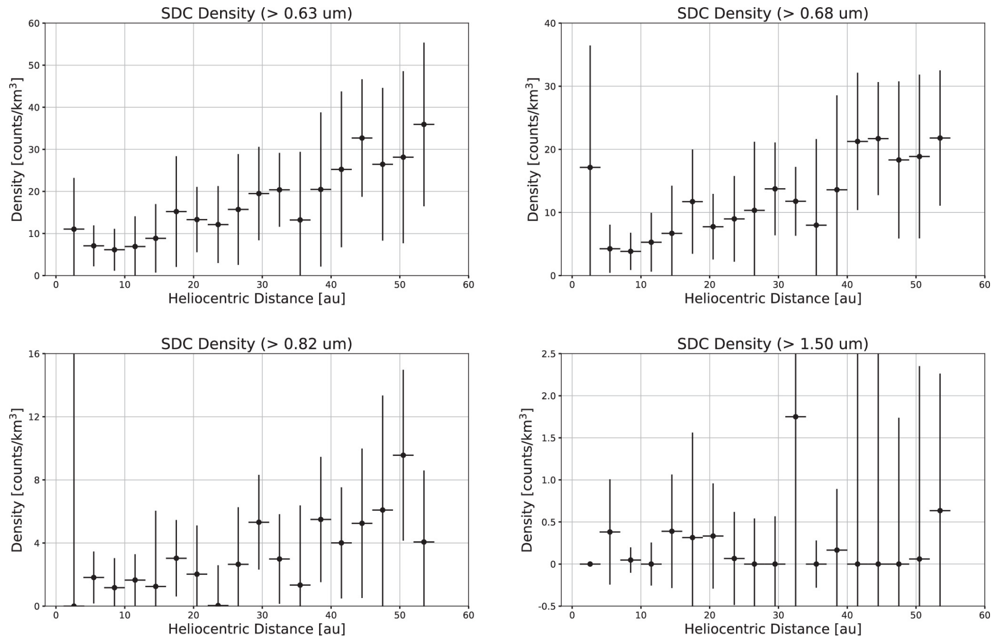
Figure 2. from Alex Doner et al 2024 Astrophys. J. Lett. 961 doi:10.3847/2041-8213/ad18b0 https://dx.doi.org/10.3847/2041-8213/ad18b0 © 2024. The Author(s). Published by the American Astronomical Society.
