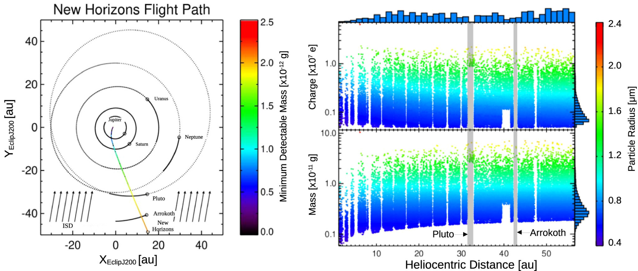
Figure 1. from Alex Doner et al 2024 Astrophys. J. Lett. 961 doi:10.3847/2041-8213/ad18b0 https://dx.doi.org/10.3847/2041-8213/ad18b0 © 2024. The Author(s). Published by the American Astronomical Society.
