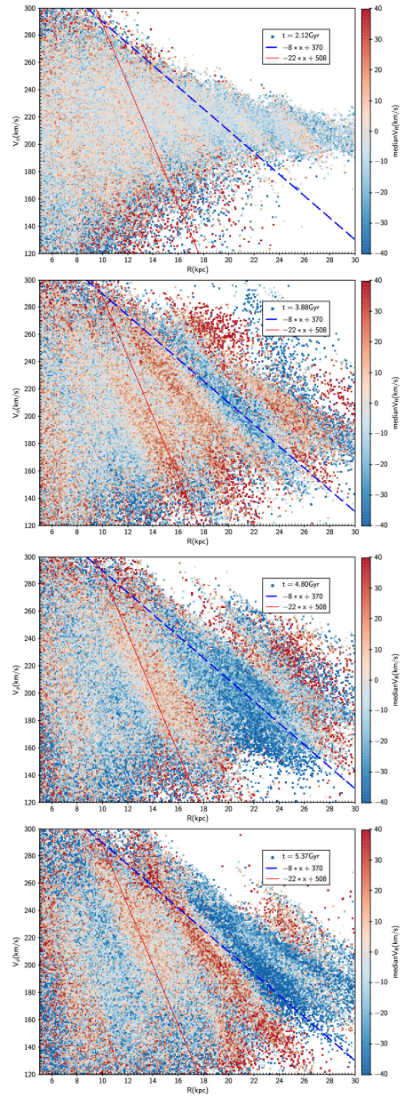
Figure 9. from Yuqin Chen et al 2024 Astrophys. J. Lett. 961 doi:10.3847/2041-8213/ad18a7 https://dx.doi.org/10.3847/2041-8213/ad18a7 © 2024. The Author(s). Published by the American Astronomical Society.
