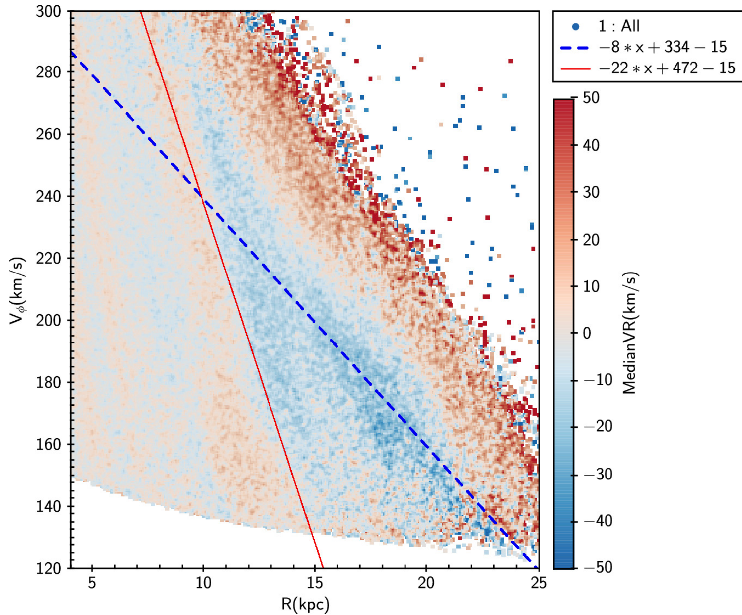
Figure 7. from Yuqin Chen et al 2024 Astrophys. J. Lett. 961 doi:10.3847/2041-8213/ad18a7 https://dx.doi.org/10.3847/2041-8213/ad18a7 © 2024. The Author(s). Published by the American Astronomical Society.
