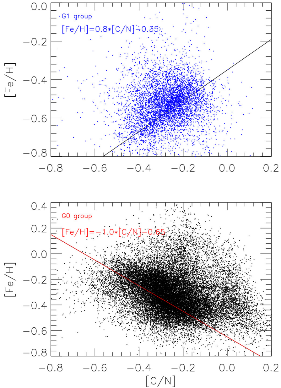
Figure 5. from Yuqin Chen et al 2024 Astrophys. J. Lett. 961 doi:10.3847/2041-8213/ad18a7 https://dx.doi.org/10.3847/2041-8213/ad18a7 © 2024. The Author(s). Published by the American Astronomical Society.
