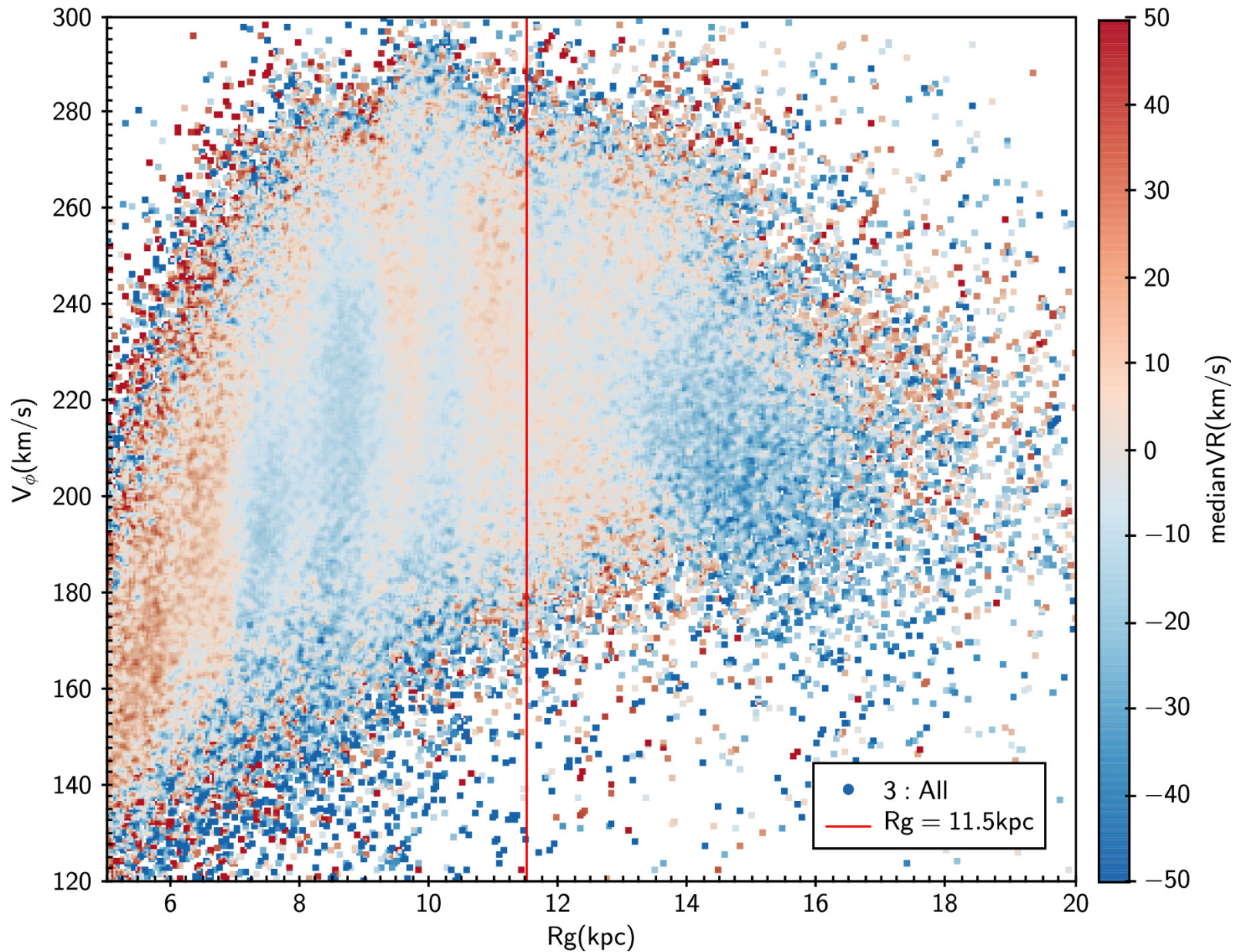
Figure 2. from Yuqin Chen et al 2024 Astrophys. J. Lett. 961 doi:10.3847/2041-8213/ad18a7 https://dx.doi.org/10.3847/2041-8213/ad18a7 © 2024. The Author(s). Published by the American Astronomical Society.
