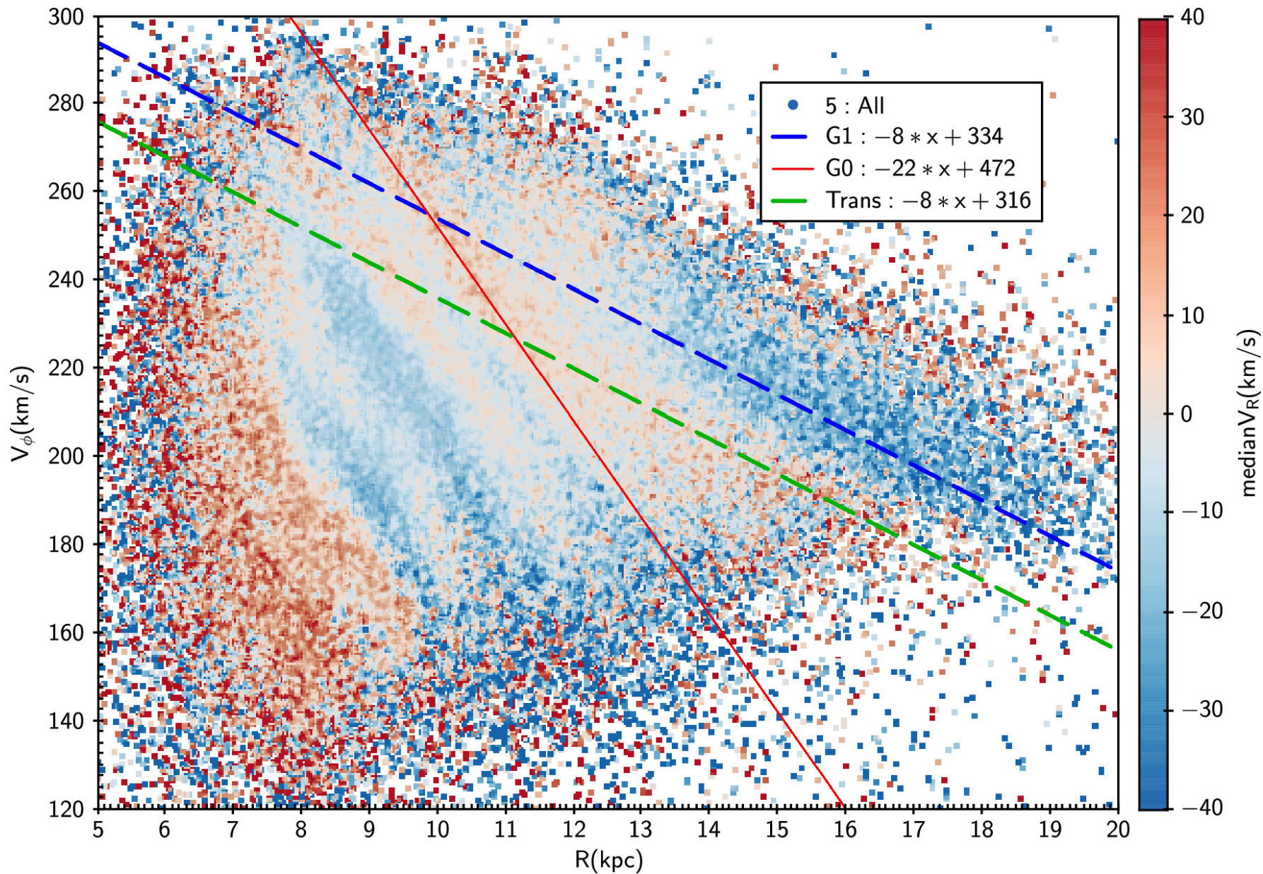
Figure 1. from Yuqin Chen et al 2024 Astrophys. J. Lett. 961 doi:10.3847/2041-8213/ad18a7 https://dx.doi.org/10.3847/2041-8213/ad18a7 © 2024. The Author(s). Published by the American Astronomical Society.
