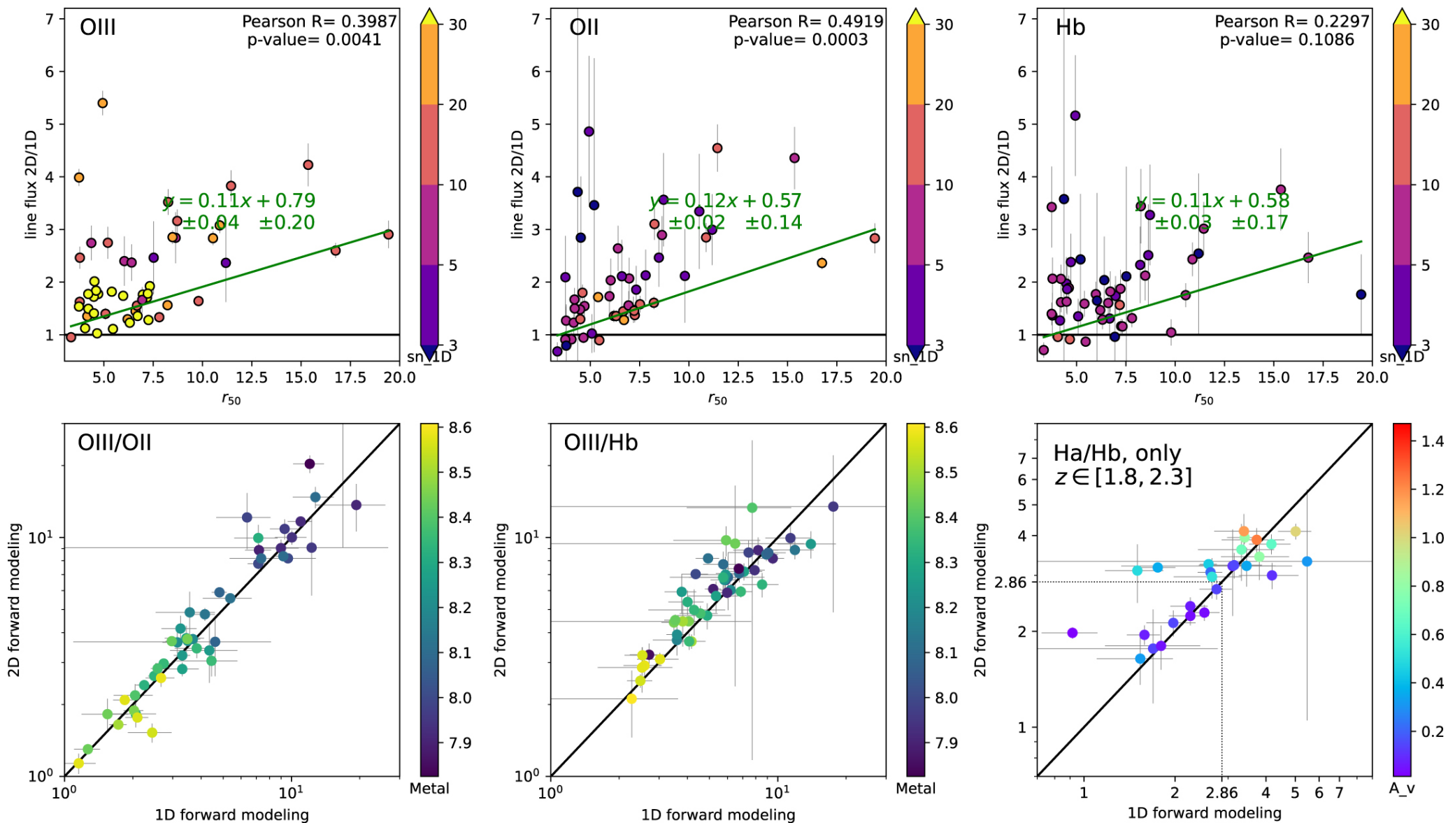
Figure 6. from Xianlong He et al 2024 Astrophys. J. Lett. 960 doi:10.3847/2041-8213/ad12cd https://dx.doi.org/10.3847/2041-8213/ad12cd © 2024. The Author(s). Published by the American Astronomical Society.
