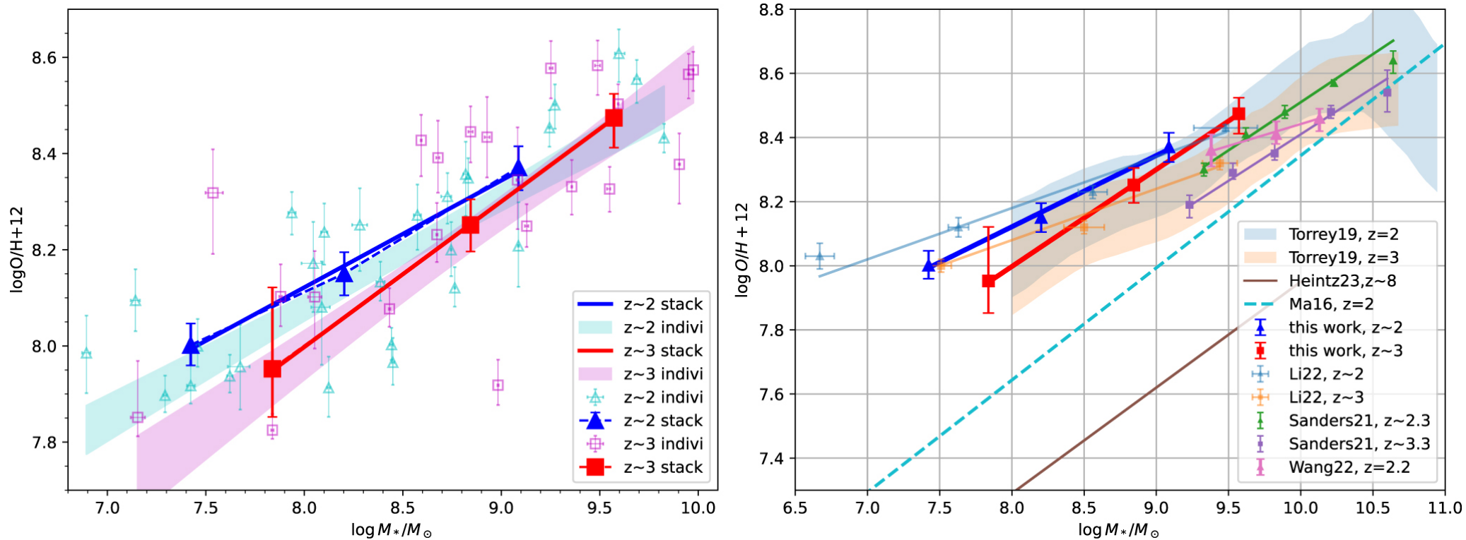
Figure 5. from Xianlong He et al 2024 Astrophys. J. Lett. 960 doi:10.3847/2041-8213/ad12cd https://dx.doi.org/10.3847/2041-8213/ad12cd © 2024. The Author(s). Published by the American Astronomical Society.
