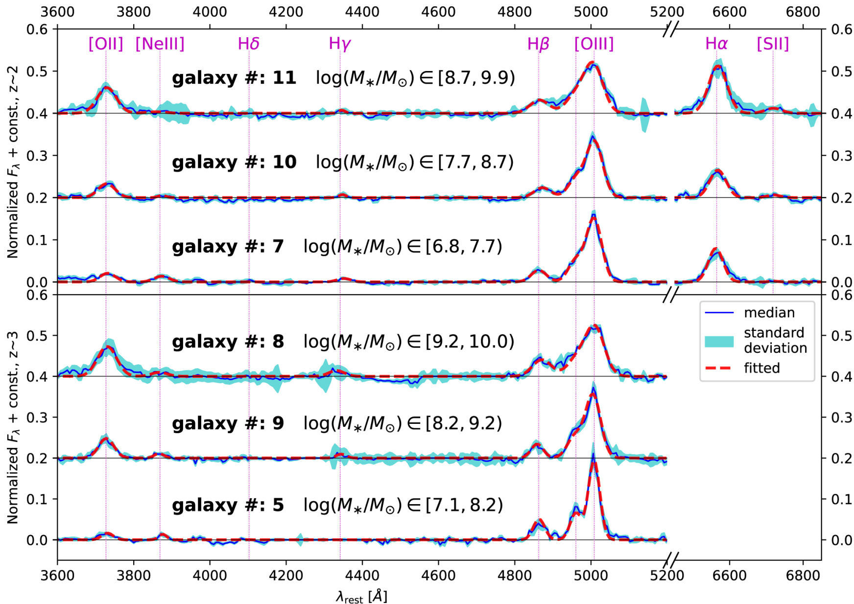
Figure 4. from Xianlong He et al 2024 Astrophys. J. Lett. 960 doi:10.3847/2041-8213/ad12cd https://dx.doi.org/10.3847/2041-8213/ad12cd © 2024. The Author(s). Published by the American Astronomical Society.
