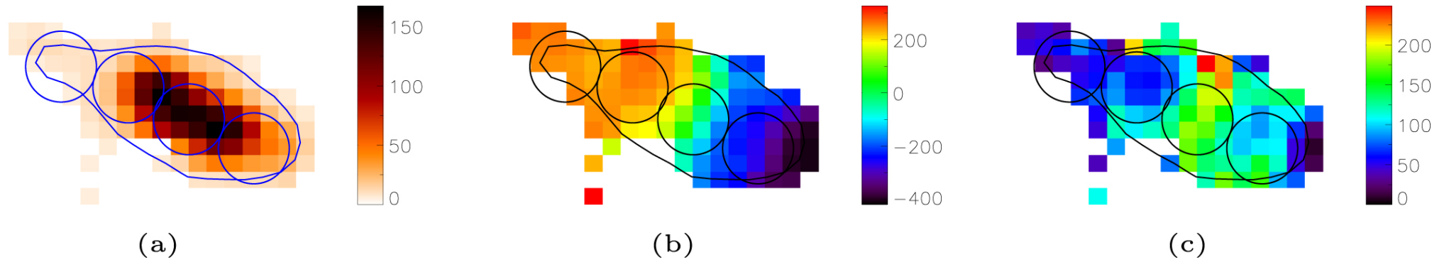
Figure 4. from Jason Young et al 2023 Astrophys. J. Lett. 958 doi:10.3847/2041-8213/ad07e1 https://dx.doi.org/10.3847/2041-8213/ad07e1 © 2023. The Author(s). Published by the American Astronomical Society.
