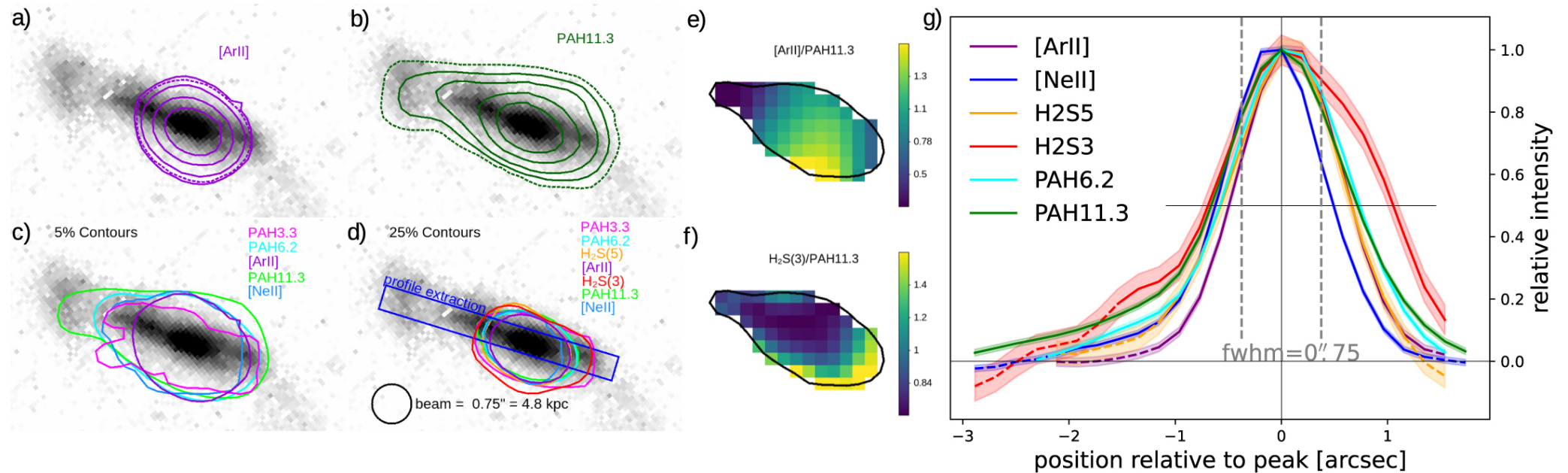
Figure 3. from Jason Young et al 2023 Astrophys. J. Lett. 958 doi:10.3847/2041-8213/ad07e1 https://dx.doi.org/10.3847/2041-8213/ad07e1 © 2023. The Author(s). Published by the American Astronomical Society.
