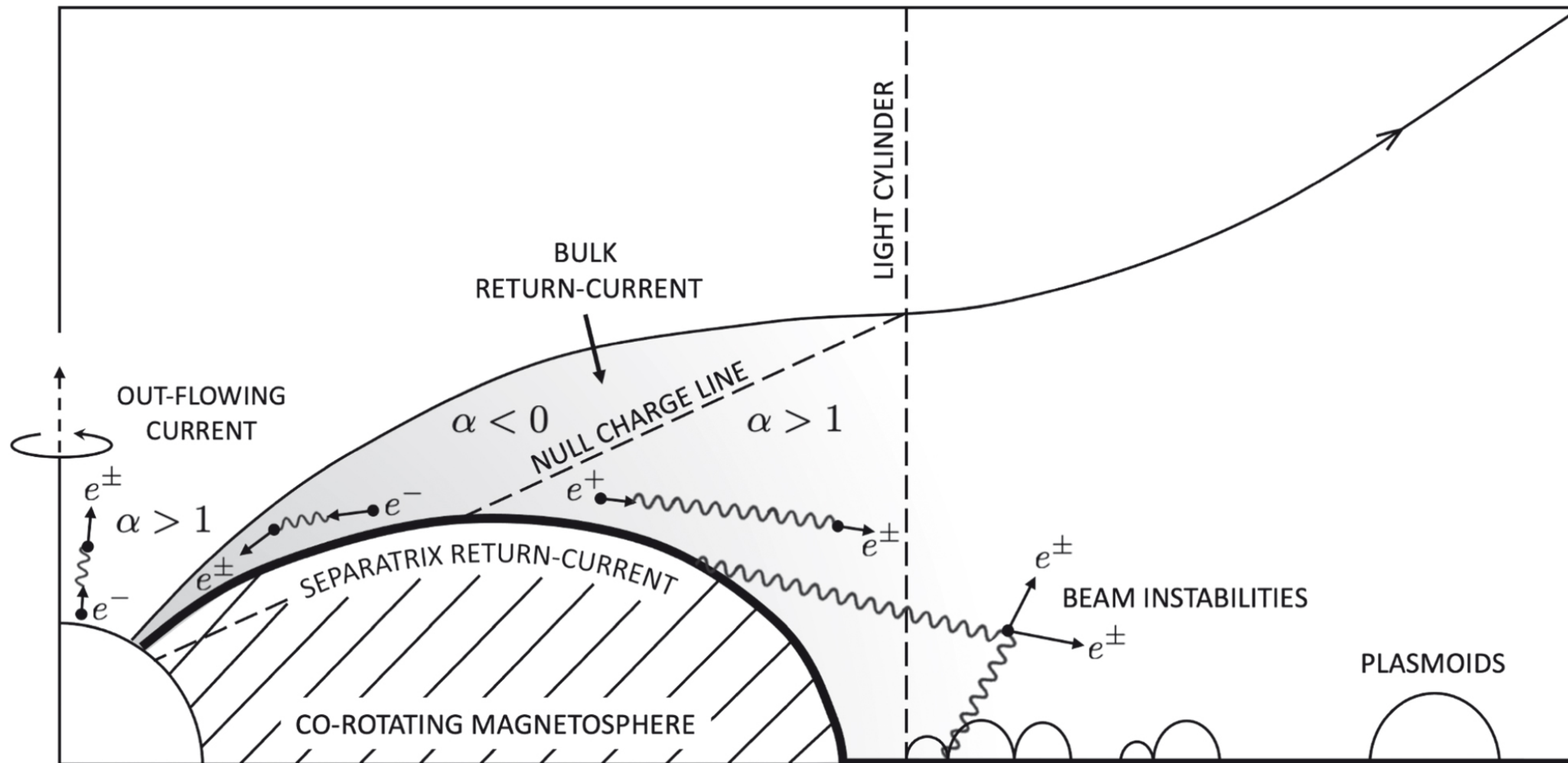
Figure 4. from Ashley Bransgrove et al 2023 Astrophys. J. Lett. 958 doi:10.3847/2041-8213/ad0556 https://dx.doi.org/10.3847/2041-8213/ad0556 © 2023. The Author(s). Published by the American Astronomical Society.
