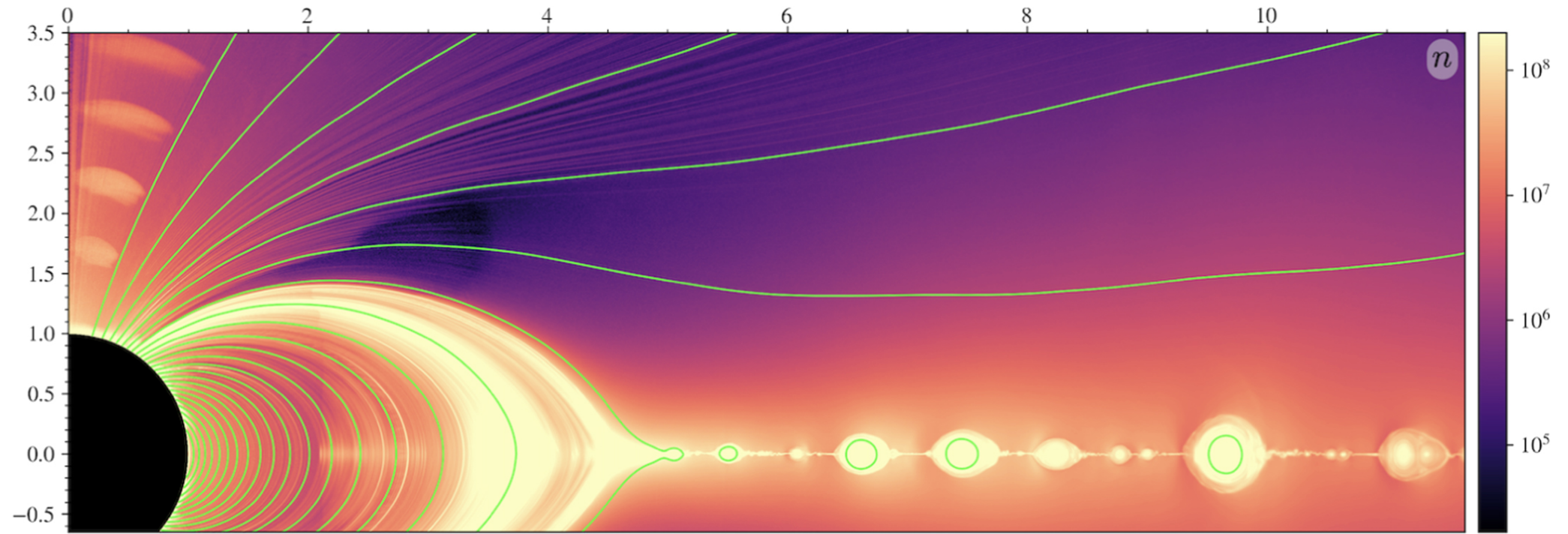
Figure 1. from Ashley Bransgrove et al 2023 Astrophys. J. Lett. 958 doi:10.3847/2041-8213/ad0556 https://dx.doi.org/10.3847/2041-8213/ad0556 © 2023. The Author(s). Published by the American Astronomical Society.
