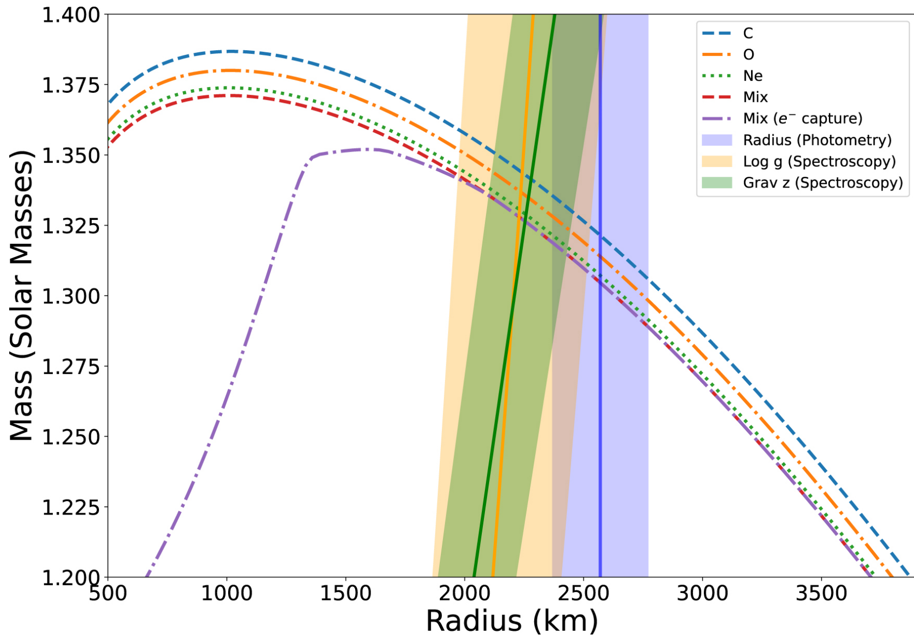
Figure 4. from David R. Miller et al 2023 Astrophys. J. Lett. 956 doi:10.3847/2041-8213/acffc4 https://dx.doi.org/10.3847/2041-8213/acffc4 © 2023. The Author(s). Published by the American Astronomical Society.
