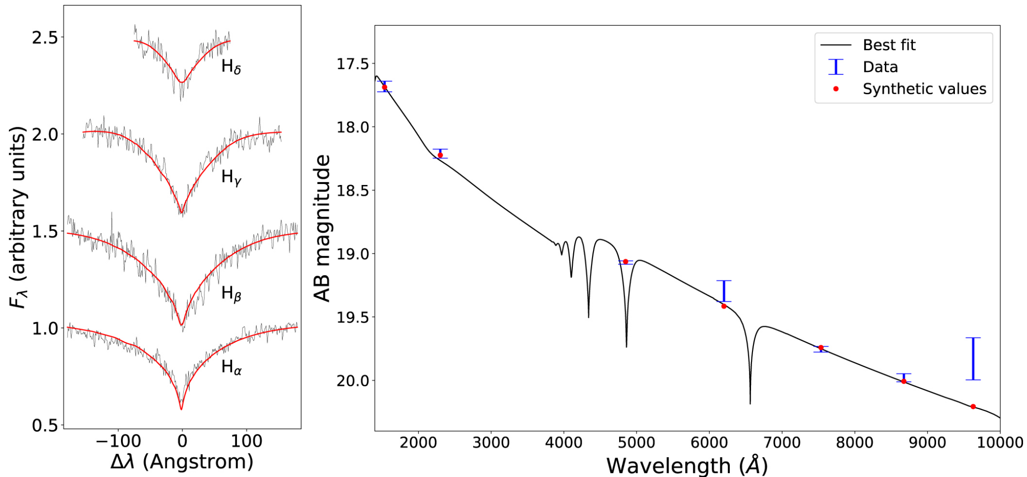
Figure 3. from David R. Miller et al 2023 Astrophys. J. Lett. 956 doi:10.3847/2041-8213/acffc4 https://dx.doi.org/10.3847/2041-8213/acffc4 © 2023. The Author(s). Published by the American Astronomical Society.
