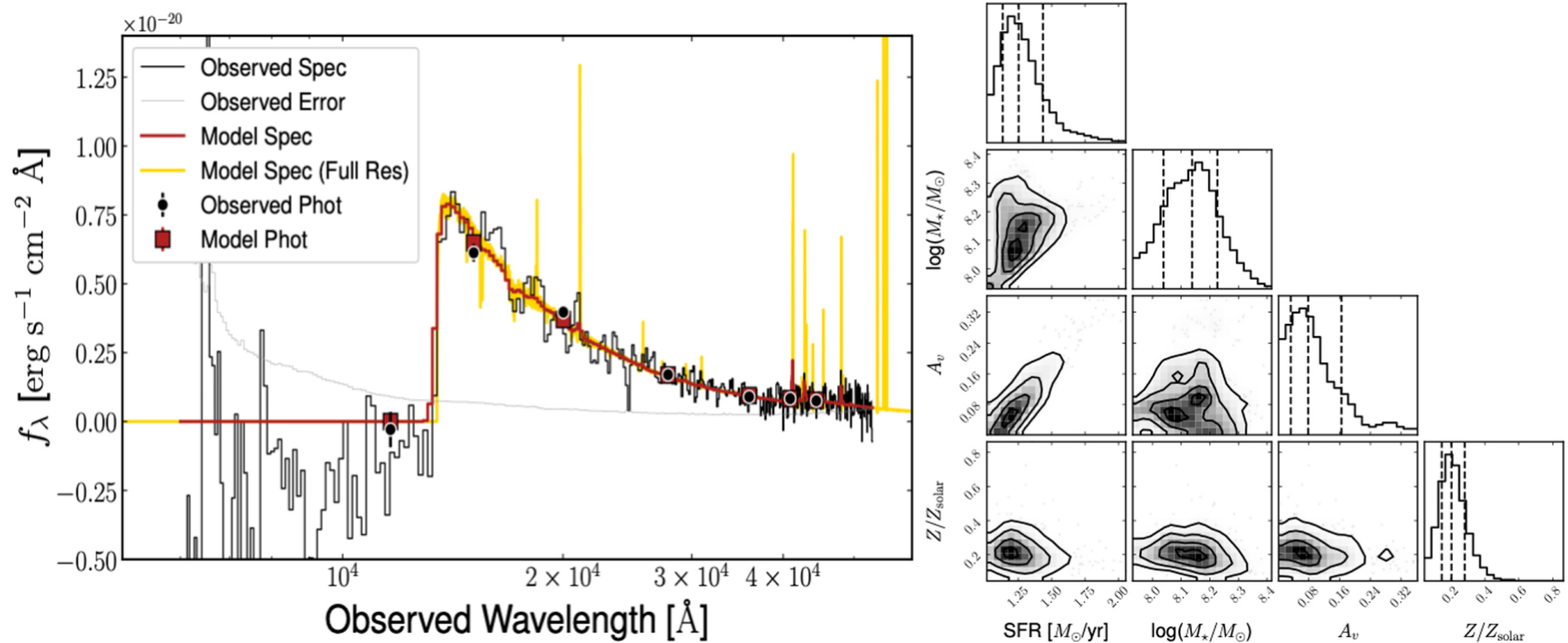
Figure 4. from Andy D. Goulding et al 2023 Astrophys. J. Lett. 955 doi:10.3847/2041-8213/acf7c5 https://dx.doi.org/10.3847/2041-8213/acf7c5 © 2023. The Author(s). Published by the American Astronomical Society.
