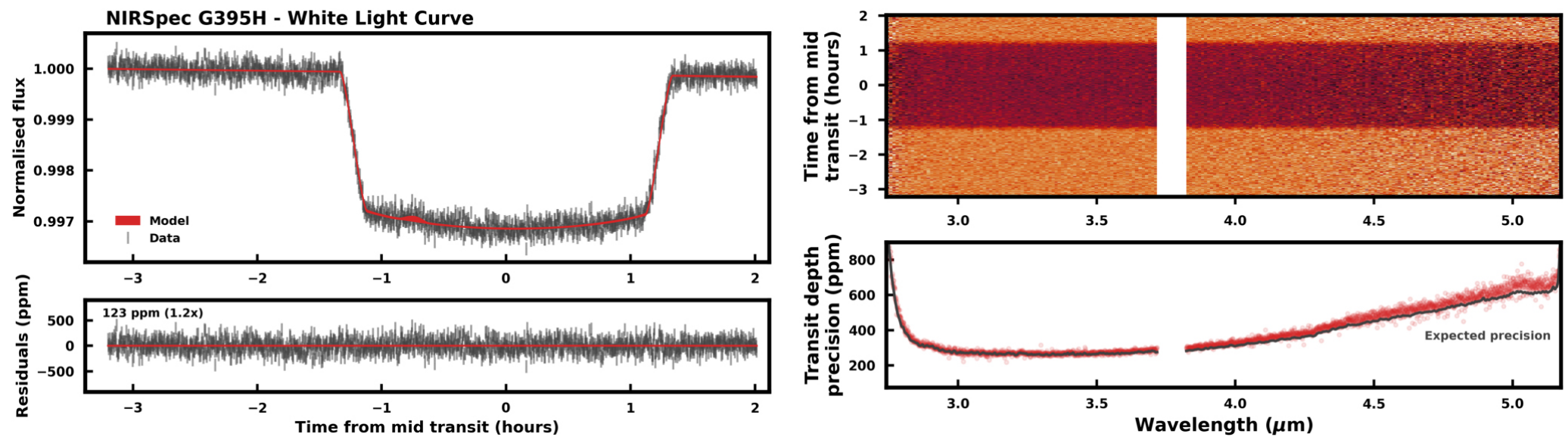
Figure 1. from Nikku Madhusudhan et al 2023 Astrophys. J. Lett. 956 doi:10.3847/2041-8213/acf577 https://dx.doi.org/10.3847/2041-8213/acf577 © 2023. The Author(s). Published by the American Astronomical Society.
