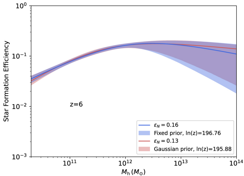
Figure 5. from Yi-Ying Wang et al 2023 Astrophys. J. Lett. 954 doi:10.3847/2041-8213/acf46c https://dx.doi.org/10.3847/2041-8213/acf46c © 2023. The Author(s). Published by the American Astronomical Society.
