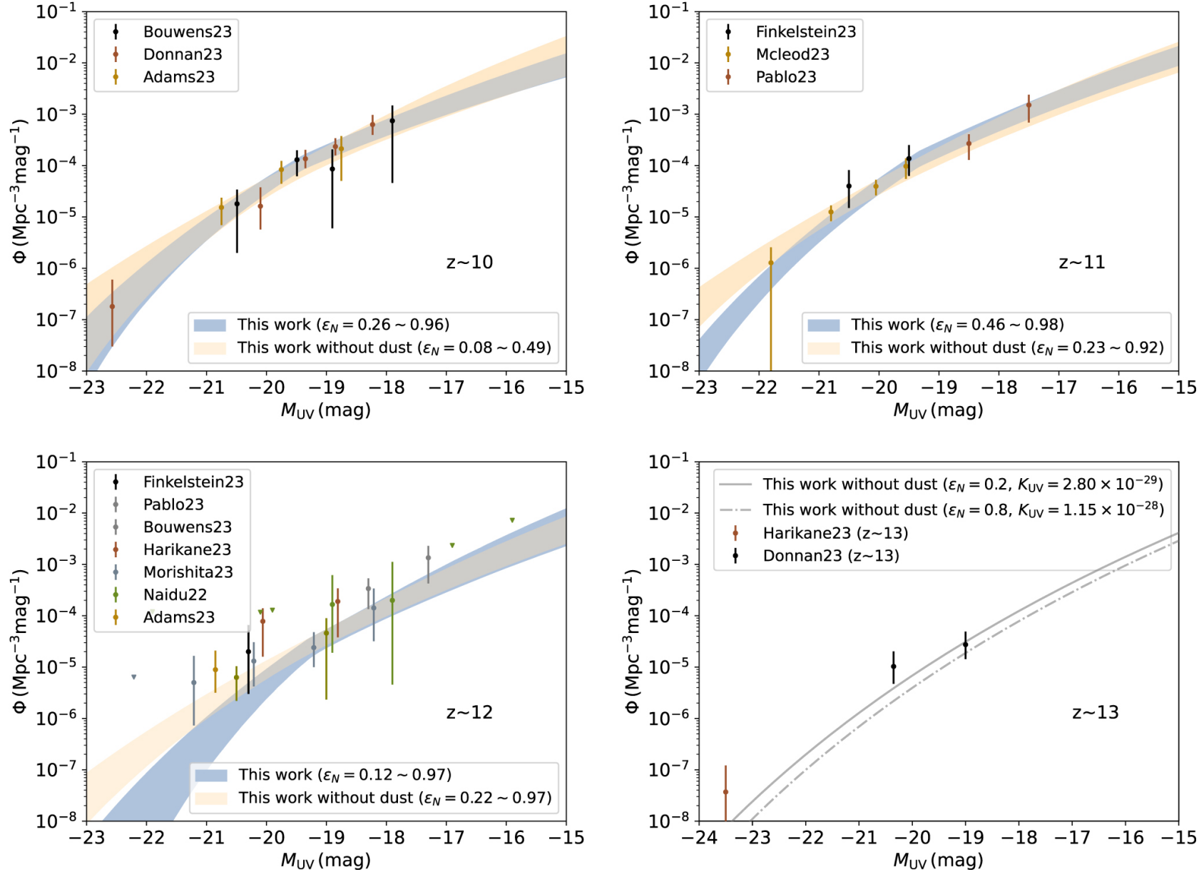
Figure 3. from Yi-Ying Wang et al 2023 Astrophys. J. Lett. 954 doi:10.3847/2041-8213/acf46c https://dx.doi.org/10.3847/2041-8213/acf46c © 2023. The Author(s). Published by the American Astronomical Society.
