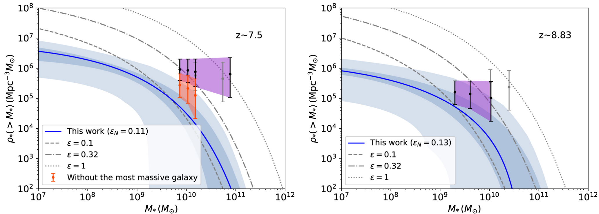
Figure 2. from Yi-Ying Wang et al 2023 Astrophys. J. Lett. 954 doi:10.3847/2041-8213/acf46c https://dx.doi.org/10.3847/2041-8213/acf46c © 2023. The Author(s). Published by the American Astronomical Society.
