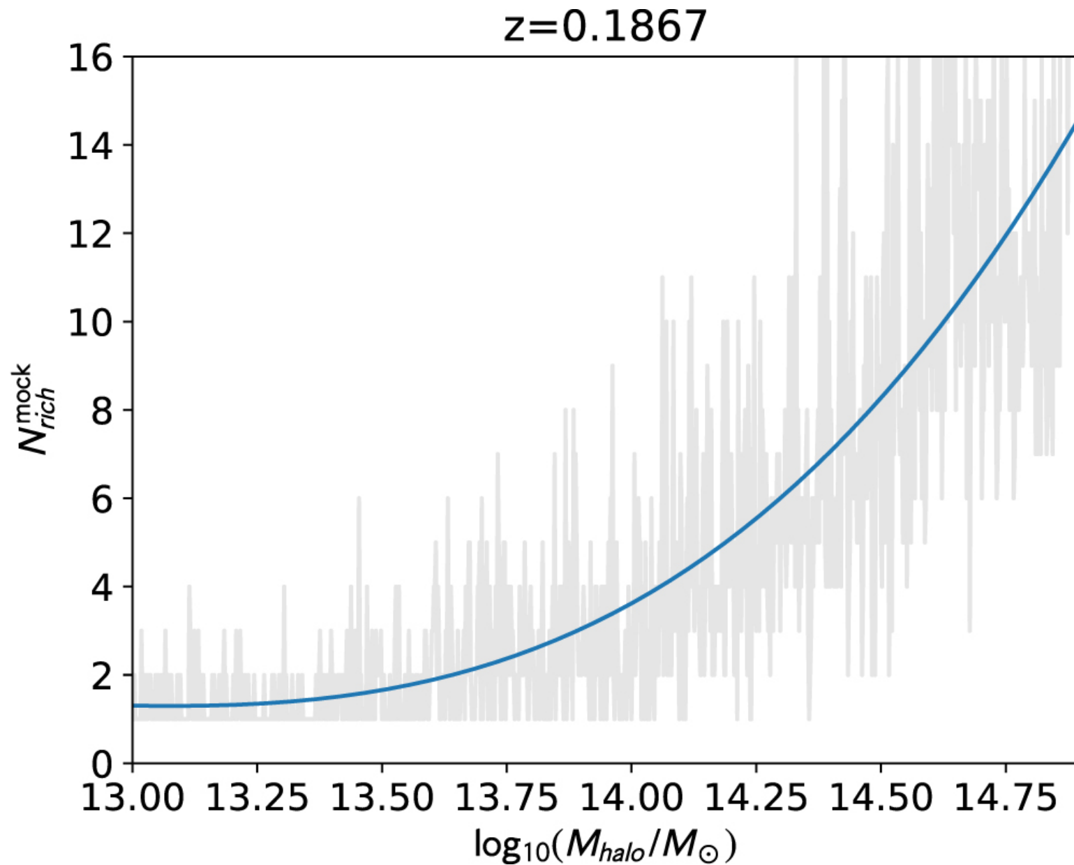
Figure 3. from Khee-Gan Lee et al 2023 Astrophys. J. Lett. 954 doi:10.3847/2041-8213/acefb5 https://dx.doi.org/10.3847/2041-8213/acefb5 © 2023. The Author(s). Published by the American Astronomical Society.
