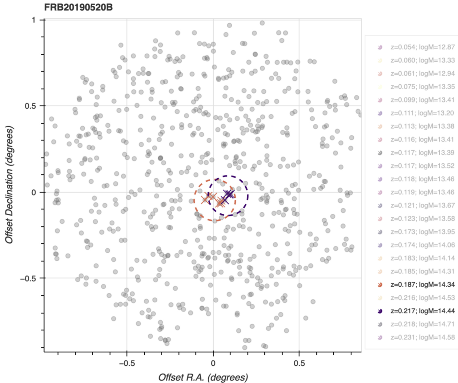
Figure 2. from Khee-Gan Lee et al 2023 Astrophys. J. Lett. 954 doi:10.3847/2041-8213/acefb5 https://dx.doi.org/10.3847/2041-8213/acefb5 © 2023. The Author(s). Published by the American Astronomical Society.
