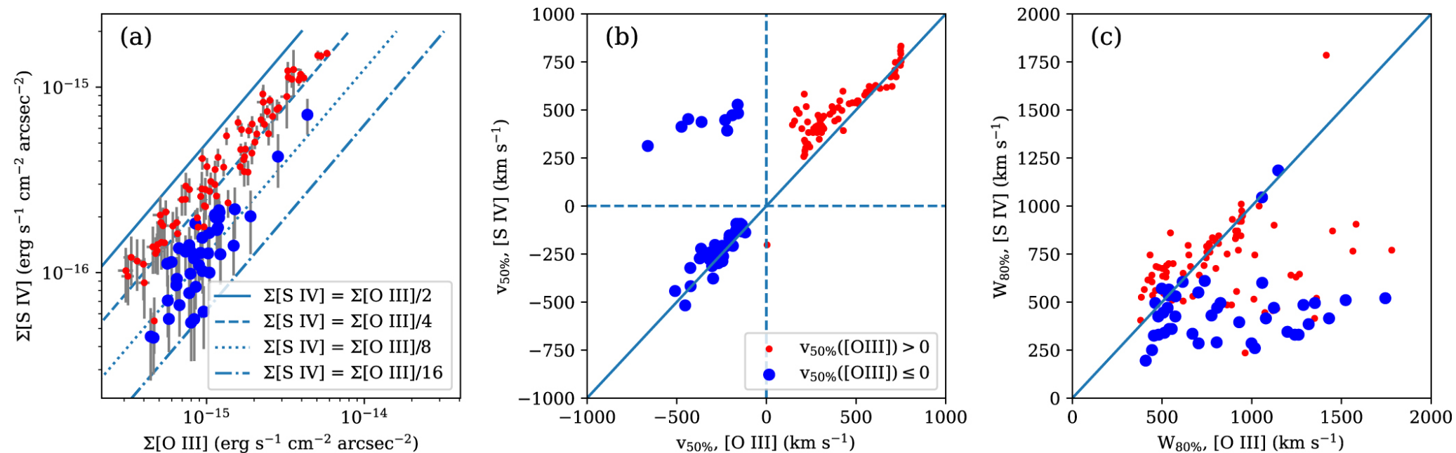
Figure 3. from David S. N. Rupke et al 2023 Astrophys. J. Lett. 953 doi:10.3847/2041-8213/aced85 https://dx.doi.org/10.3847/2041-8213/aced85 © 2023. The Author(s). Published by the American Astronomical Society.
