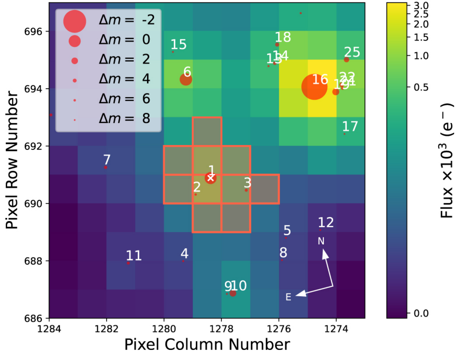
Figure 2. from Ismael Mireles et al 2023 Astrophys. J. Lett. 954 doi:10.3847/2041-8213/aceb69 https://dx.doi.org/10.3847/2041-8213/aceb69 © 2023. The Author(s). Published by the American Astronomical Society.
