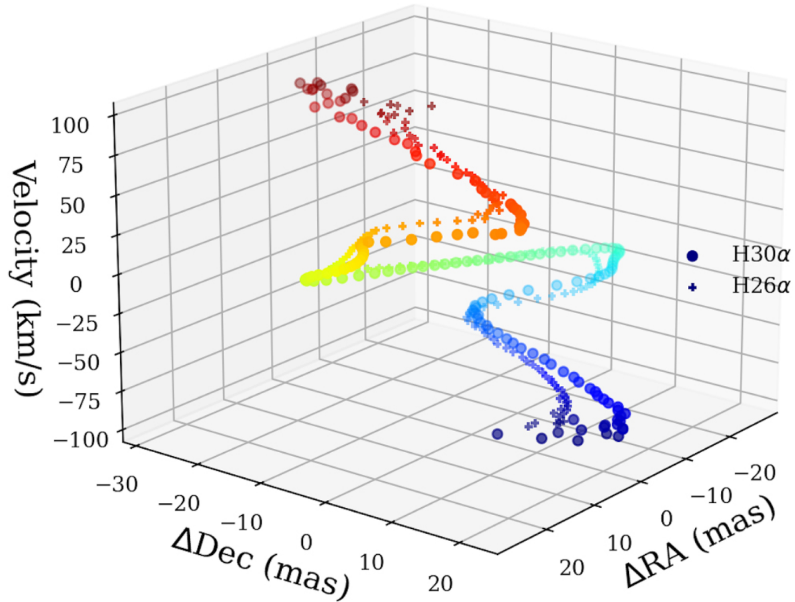
Figure 5. from Sirina Prasad et al 2023 Astrophys. J. Lett. 953 doi:10.3847/2041-8213/ace7ba https://dx.doi.org/10.3847/2041-8213/ace7ba © 2023. The Author(s). Published by the American Astronomical Society.
