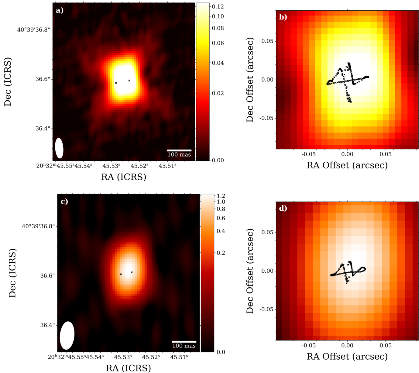
Figure 1. from Sirina Prasad et al 2023 Astrophys. J. Lett. 953 doi:10.3847/2041-8213/ace7ba https://dx.doi.org/10.3847/2041-8213/ace7ba © 2023. The Author(s). Published by the American Astronomical Society.
