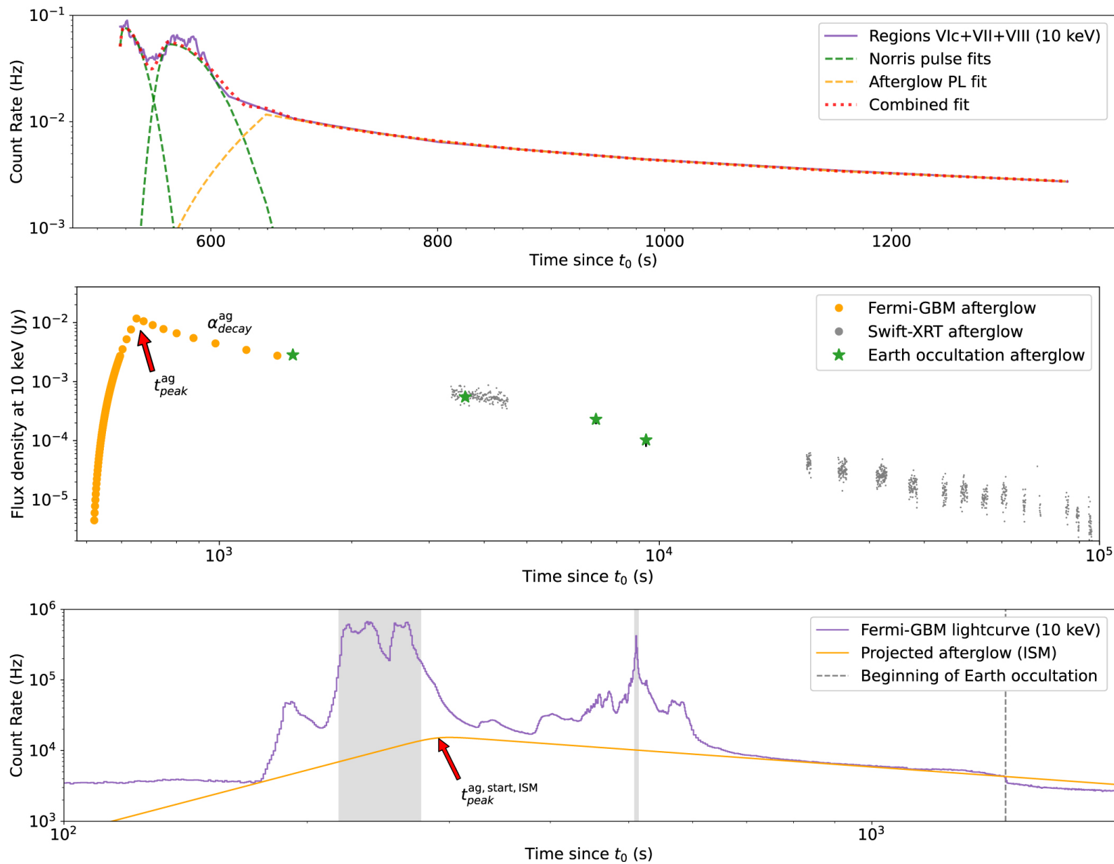
Figure 6. from S. Lesage et al 2023 Astrophys. J. Lett. 952 doi:10.3847/2041-8213/ace5b4 https://dx.doi.org/10.3847/2041-8213/ace5b4 © 2023. The Author(s). Published by the American Astronomical Society.
