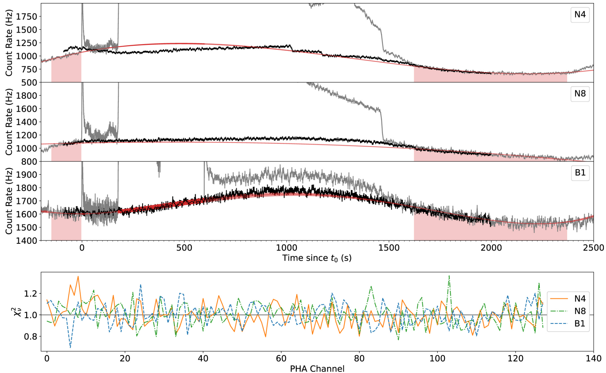
Figure 3. from S. Lesage et al 2023 Astrophys. J. Lett. 952 doi:10.3847/2041-8213/ace5b4 https://dx.doi.org/10.3847/2041-8213/ace5b4 © 2023. The Author(s). Published by the American Astronomical Society.
