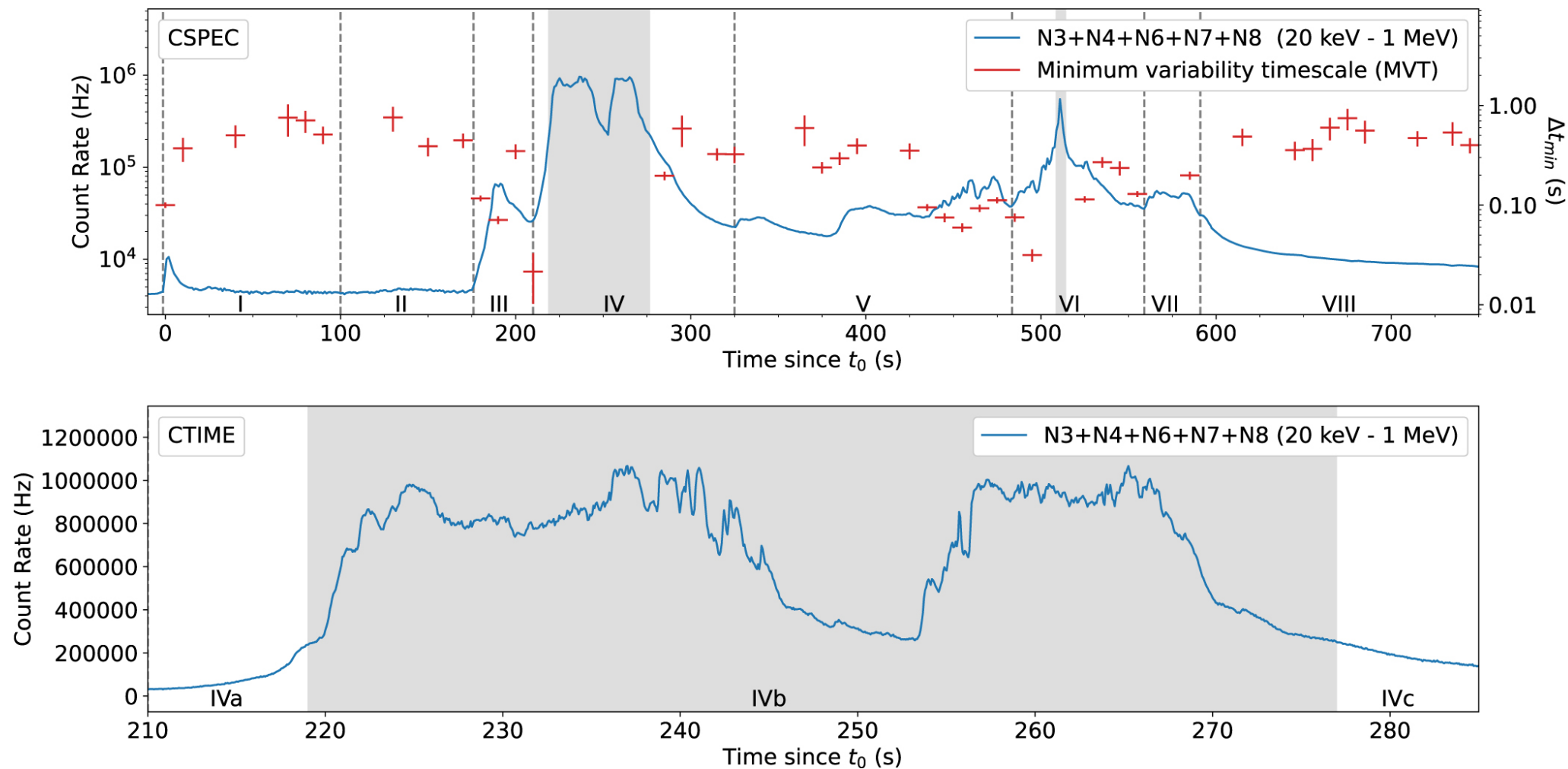
Figure 2. from S. Lesage et al 2023 Astrophys. J. Lett. 952 doi:10.3847/2041-8213/ace5b4 https://dx.doi.org/10.3847/2041-8213/ace5b4 © 2023. The Author(s). Published by the American Astronomical Society.
