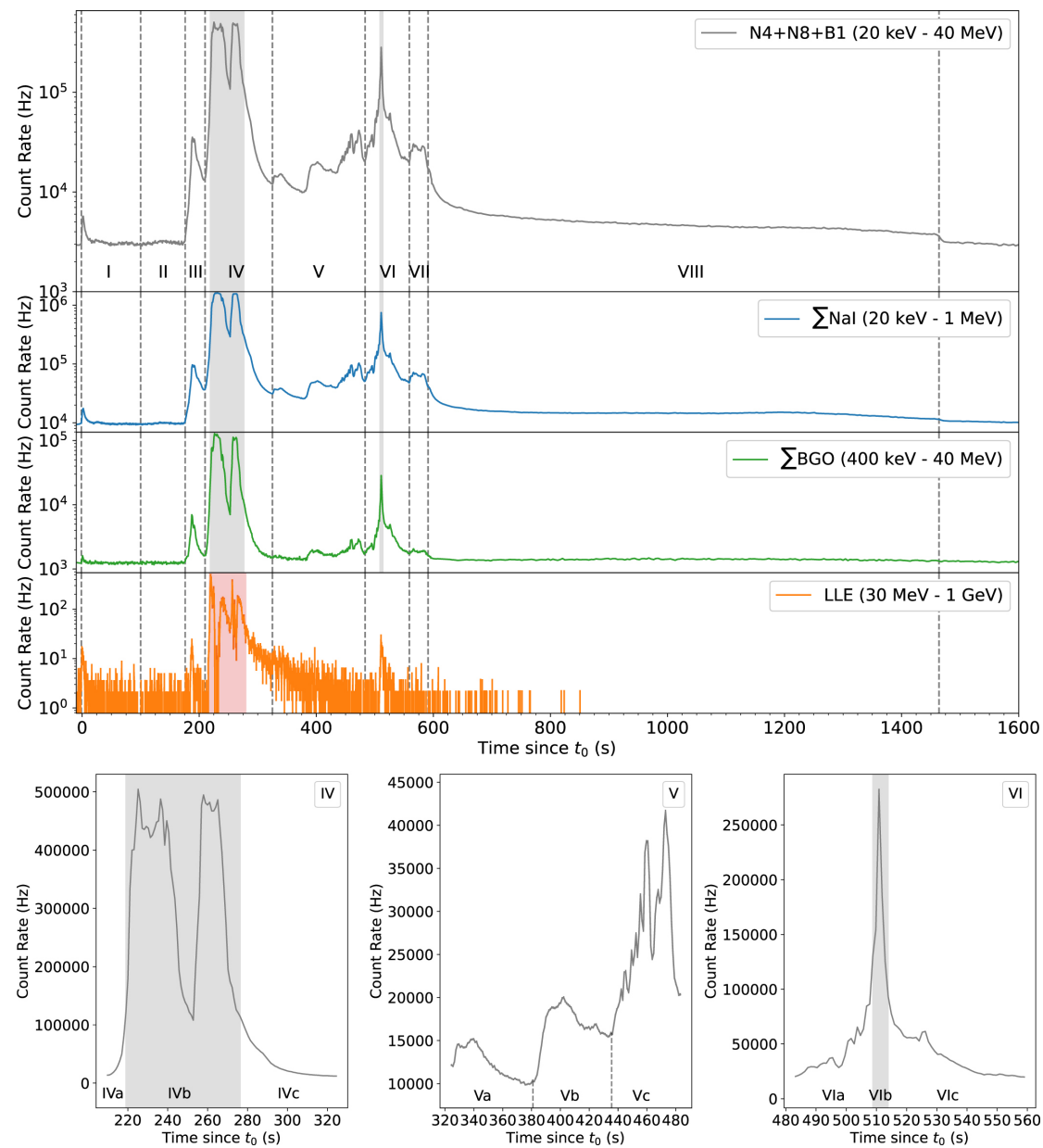
Figure 1. from S. Lesage et al 2023 Astrophys. J. Lett. 952 doi:10.3847/2041-8213/ace5b4 https://dx.doi.org/10.3847/2041-8213/ace5b4 © 2023. The Author(s). Published by the American Astronomical Society.
