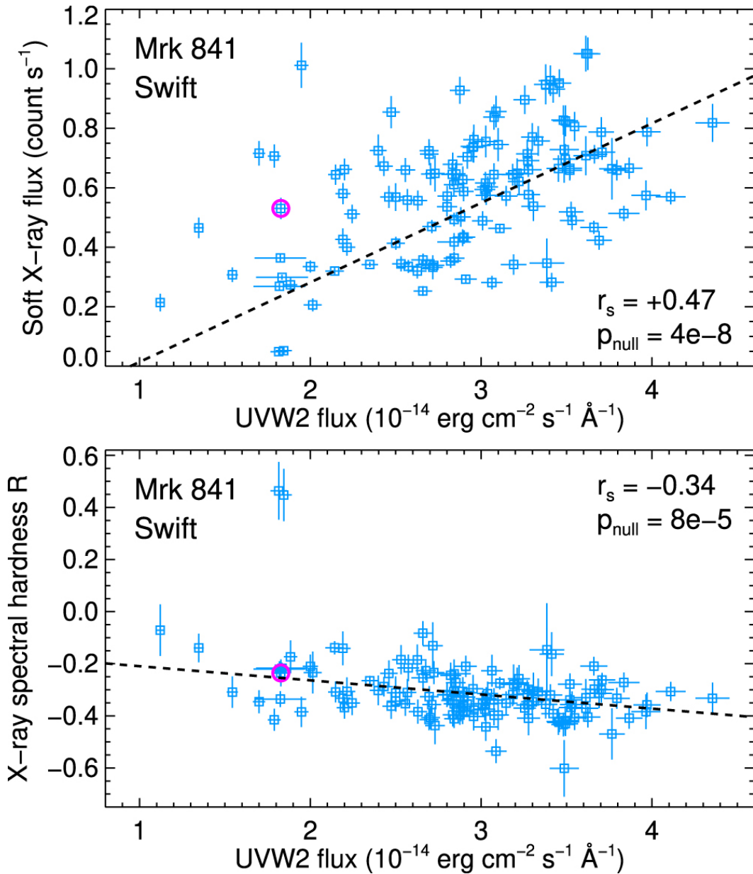
Figure 4. from Missagh Mehdipour et al 2023 Astrophys. J. Lett. 952 doi:10.3847/2041-8213/ace053 https://dx.doi.org/10.3847/2041-8213/ace053 © 2023. The Author(s). Published by the American Astronomical Society.
