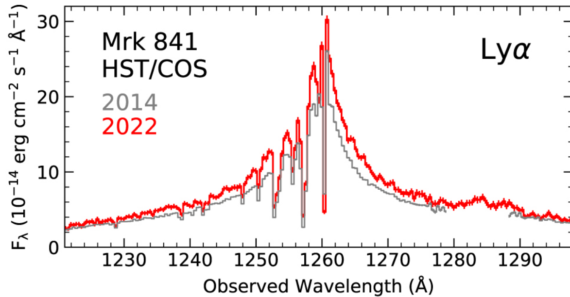
Figure 3. from Missagh Mehdipour et al 2023 Astrophys. J. Lett. 952 doi:10.3847/2041-8213/ace053 https://dx.doi.org/10.3847/2041-8213/ace053 © 2023. The Author(s). Published by the American Astronomical Society.
