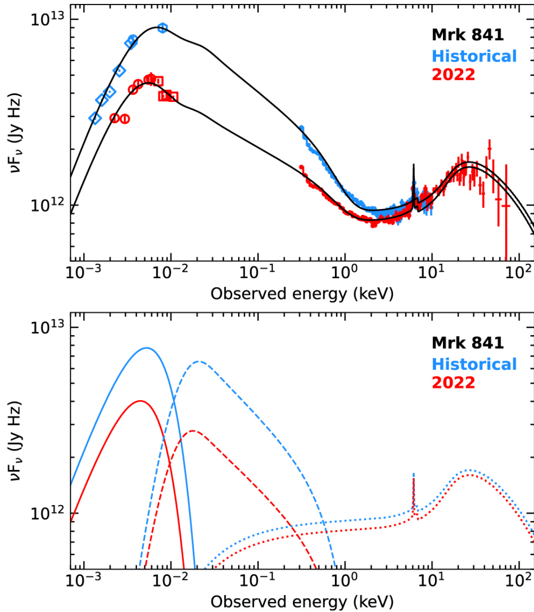
Figure 2. from Missagh Mehdipour et al 2023 Astrophys. J. Lett. 952 doi:10.3847/2041-8213/ace053 https://dx.doi.org/10.3847/2041-8213/ace053 © 2023. The Author(s). Published by the American Astronomical Society.
