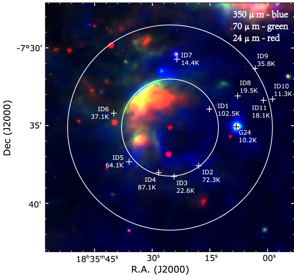
Figure 3. from Jun-Ting Liu et al 2023 Astrophys. J. Lett. 951 doi:10.3847/2041-8213/acdf5b https://dx.doi.org/10.3847/2041-8213/acdf5b © 2023. The Author(s). Published by the American Astronomical Society.
