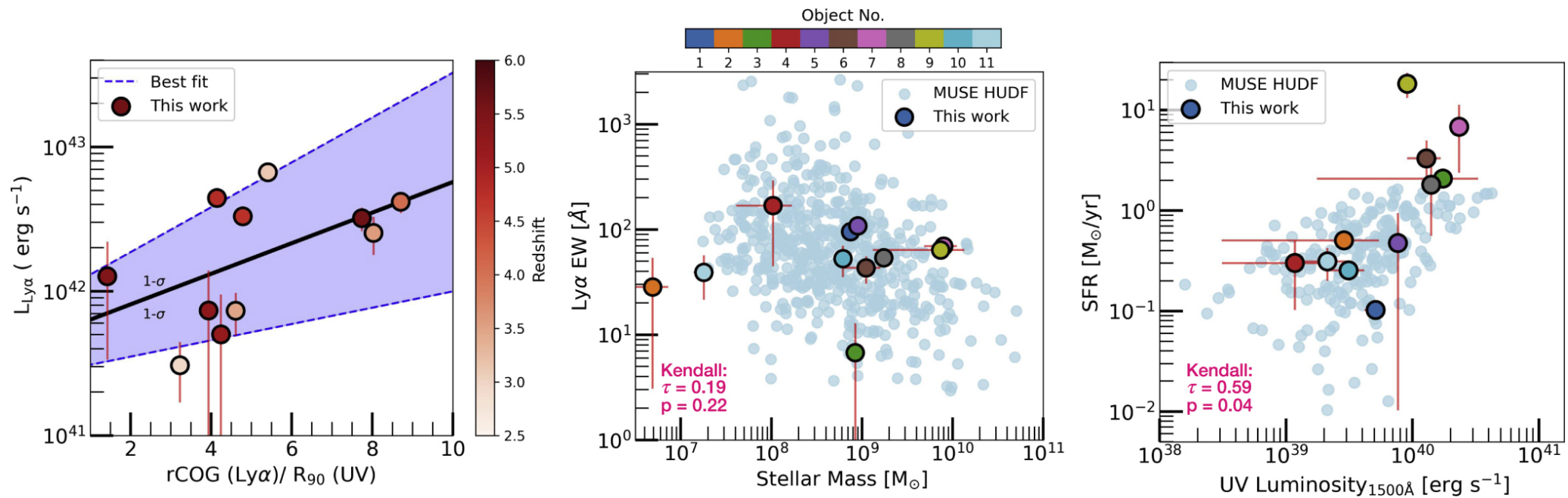
Figure 3. from Namrata Roy et al 2023 Astrophys. J. Lett. 952 doi:10.3847/2041-8213/acdbce https://dx.doi.org/10.3847/2041-8213/acdbce © 2023. The Author(s). Published by the American Astronomical Society.
