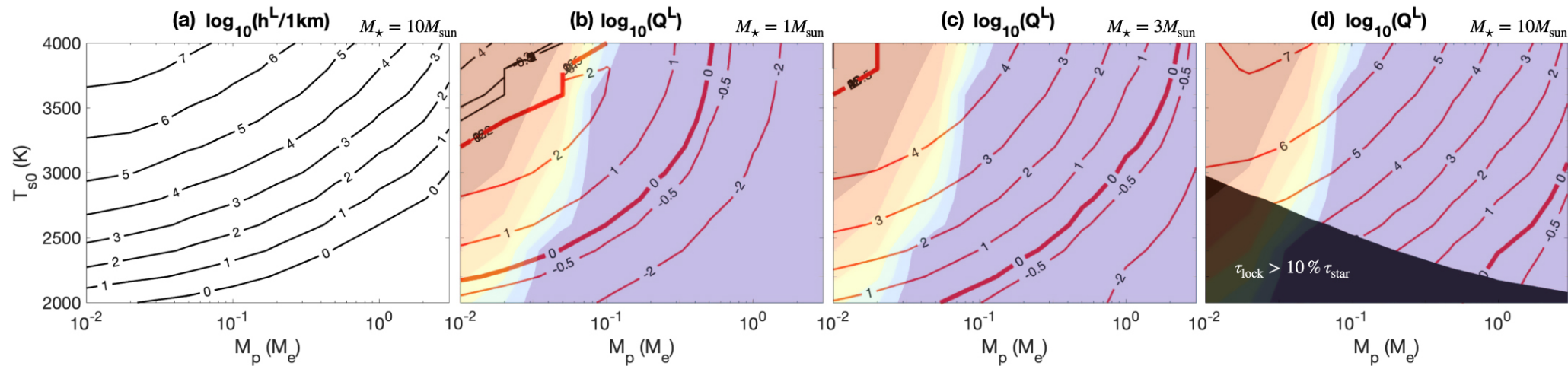
Figure 2. from Wanying Kang et al 2023 Astrophys. J. Lett. 949 doi:10.3847/2041-8213/acd691 https://dx.doi.org/10.3847/2041-8213/acd691 © 2023. The Author(s). Published by the American Astronomical Society.
