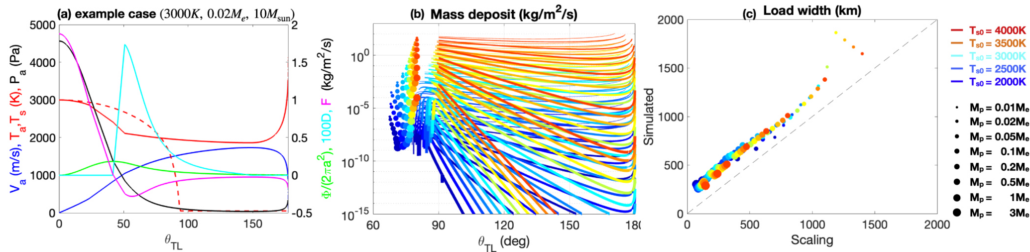
Figure 1. from Wanying Kang et al 2023 Astrophys. J. Lett. 949 doi:10.3847/2041-8213/acd691 https://dx.doi.org/10.3847/2041-8213/acd691 © 2023. The Author(s). Published by the American Astronomical Society.
